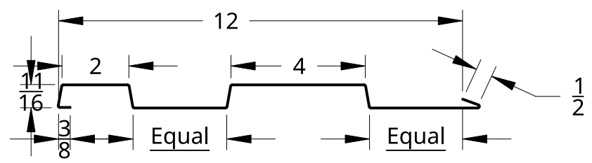
Unequal battens, 2" minimum, 5" maximum
