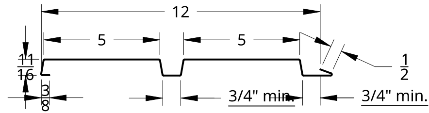
Equal battens, 2" minimum, 5" maximum
